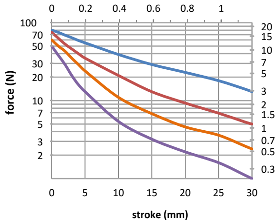
force / stroke 380 stroke (inch)
